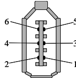
Figure 1: IEEE-1394 connector pin configuration
