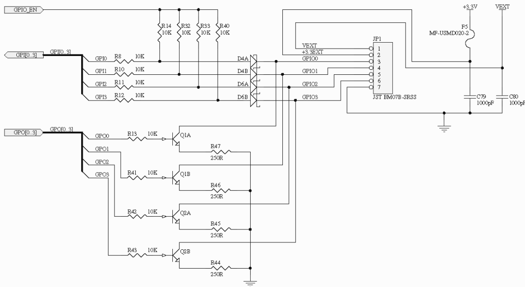
Figure 3: Firefly MV GPIO Circuit Diagram
