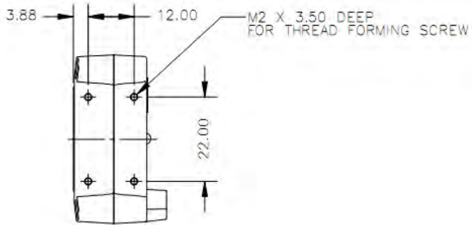
Top View with USB Connector
