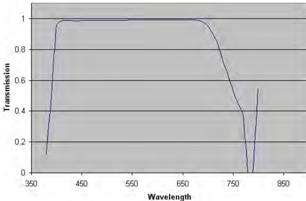
Figure 1: IR filter transmittance graph
