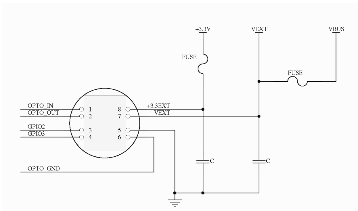
Figure 3.5: GPIO and Power Input Circuit (FL3-FW-14S3 and FL3-FW-20S4 Only)
